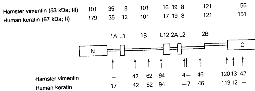
FIG. 4. Comparative structures of the human 67-kDa keratin and hamster vimentin genes. Roman numerals (II and III) refer to \alpha -helix types. The conserved secondary structure of the proteins consists of the end-domains N and C and the central \alpha -helical domain. The latter is subdivided into the 4 coiled-coil subdomains 1A, 1B, 2A, and 2B (boxes) by the non-coiled-coil linkers L1, L12, and L2. The coiled-coil subdomain 2B has a heptad polarity discontinuity (stutter) where shown. Above is shown the number of amino acid residues in each domain or subdomain of the two proteins. Below are arrows that delineate positions of introns in the genes. Numbers below refer to the amino acid number within the subdomain or C end-domain.
