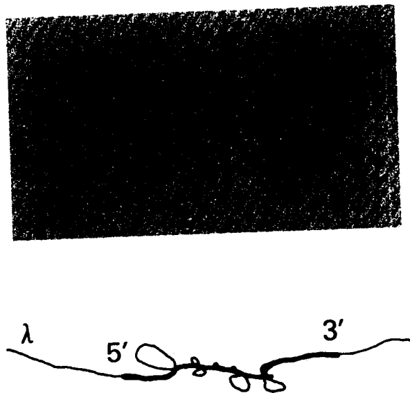
FIG. 1. R-loop analysis of the genomic clone c55 for the 67-kDa keratin gene. By this method, eight loops of intron sequences can be identified over a total estimated length of about 6.5 kbp. (Upper) Electron micrograph. ( \times 11,200 .) (Lower) Representation shows the 5' and 3' ends of the gene within the \lambda clone.
