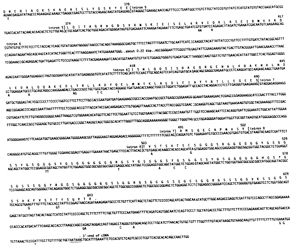
FIG. 3. DNA and amino acid sequences of the gene for the 67-kDa keratin. Regions encoded by the cDNA described elsewhere are indicated. Introns 1 and 6 were incompletely sequenced, but their sizes were estimated from the mobilities of DNA fragments of known size. The Kpn I-Fnu4HI fragment used for primer extension is shown, and the sequence extended in the experiment is indicated by the dotted line (nucleotide positions 686-758). The possible "CAT box" and likely "TATA box," "cap site," initiation codon, and polyadenylation signal sequences are underlined. The occasional nucleotides shown below the line are those that differ from the cDNA clone. The deduced amino acid sequence of 643 amino acids is shown above the nucleotide sequence, using the single-letter code (33).
