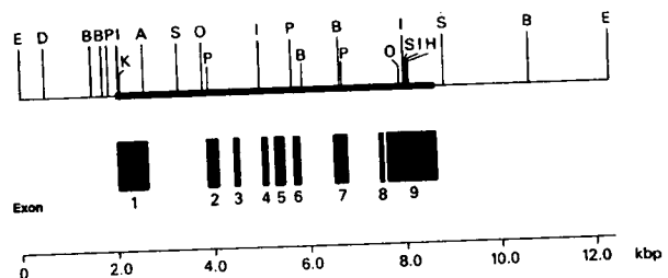
FIG. 2. Physical map of genomic clone c55 (12.3 kbp) and gene (6.25 kbp). The locations of prominent restriction endonuclease sites are shown: A, Ava I; B, Bgl II; D, Nde I; E, Eco RI; H, Bam HI; I, Nci I; K, Kpn I; O, Nco I; P, Pst I; S, Sac I. The region encoding the gene is shown by the heavy line. The nine exons representing 2.44 kb of the mRNA are shown by the black boxes.
